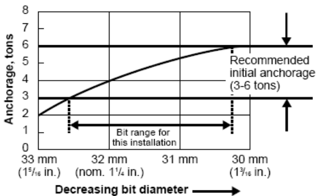
(a) Anchorage versus bit diameter
