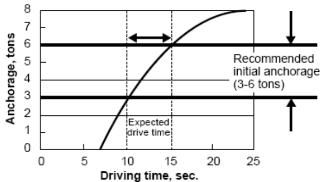
(b) Anchorage versus driving time
